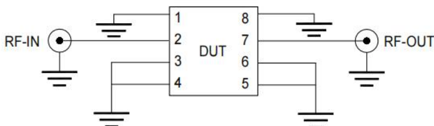
Fig 1. Block Diagram of Test Circuit used for characterization. Die is packaged in 2x2mm, 8-lead MCLP and soldered on testboard TB-1041-5-63+
