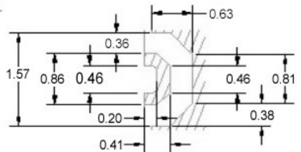
DETAIL A (2 PLACES)
