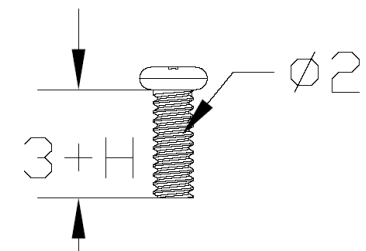
Recommended length of the screw Fig 5
