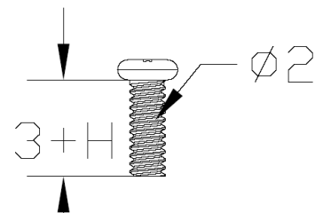
Recommended length of the screw Fig 5
