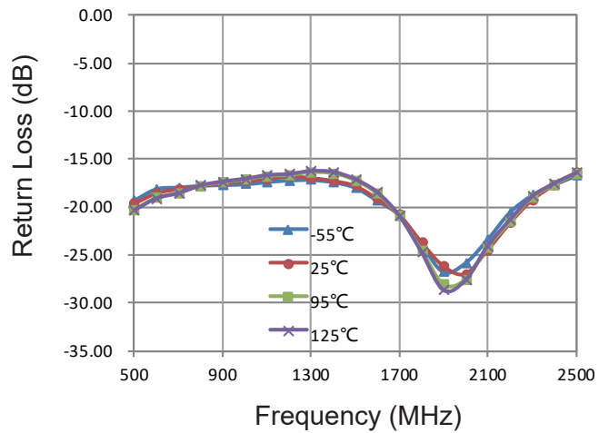
Return Loss (Port 2)
