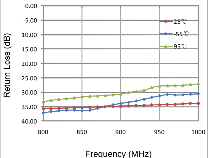
Return Loss (Port 4)
